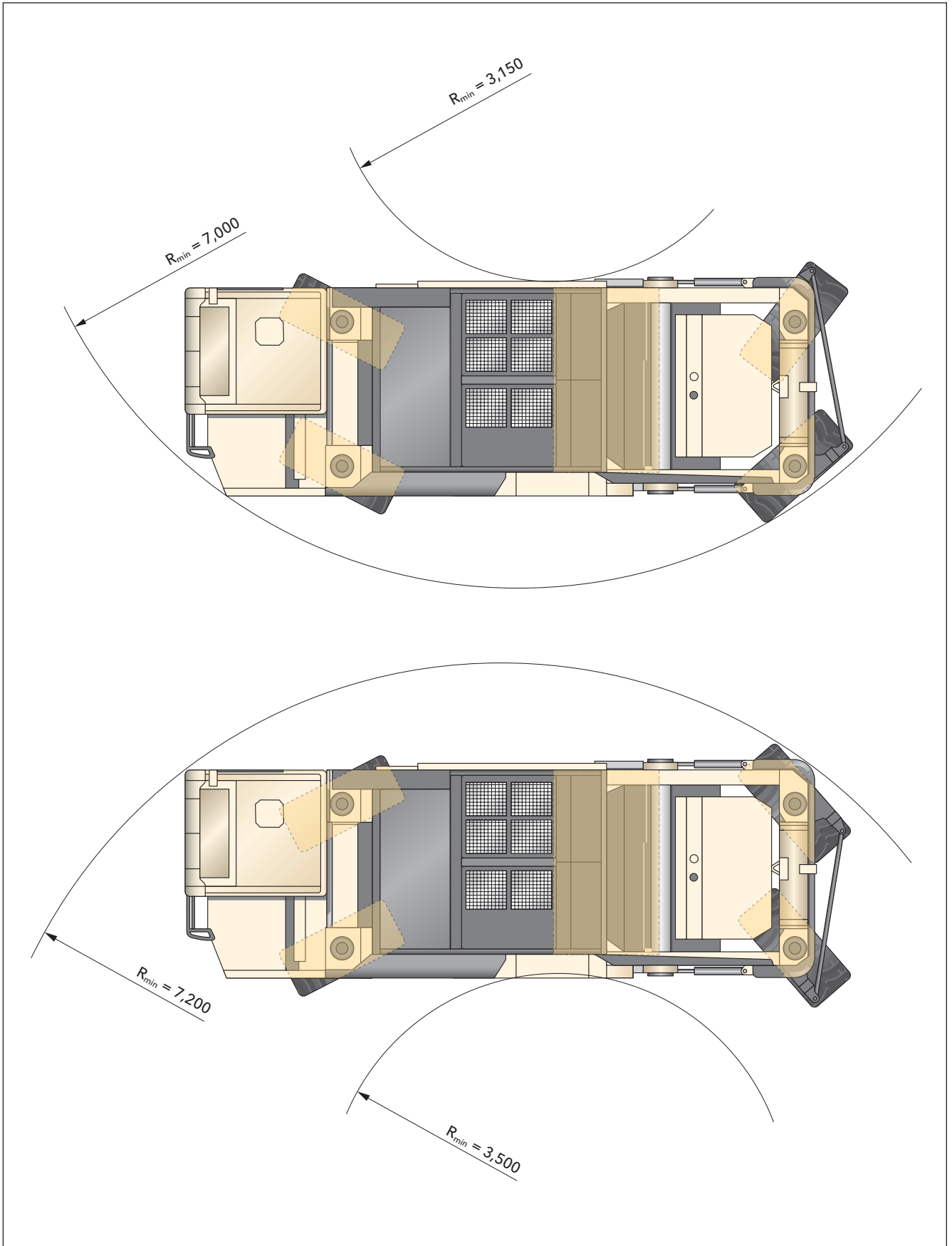
Turning radius of WR 200/WR 200i, WR 240/WR 240i and WR 250 Dimensions in mm
