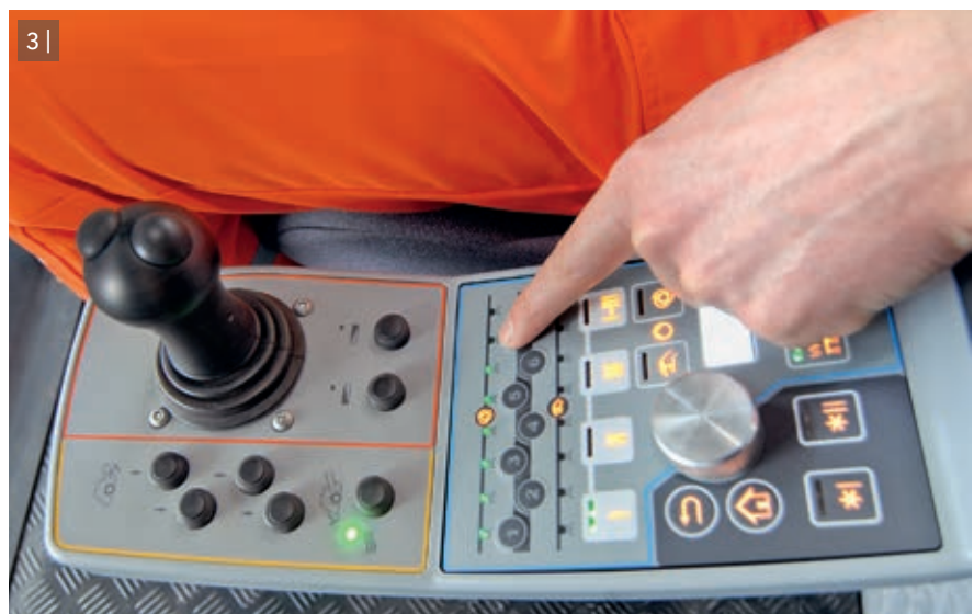
3 | Parameters such as the spraying width and amounts of binder to be added can be adjusted intuitively.
